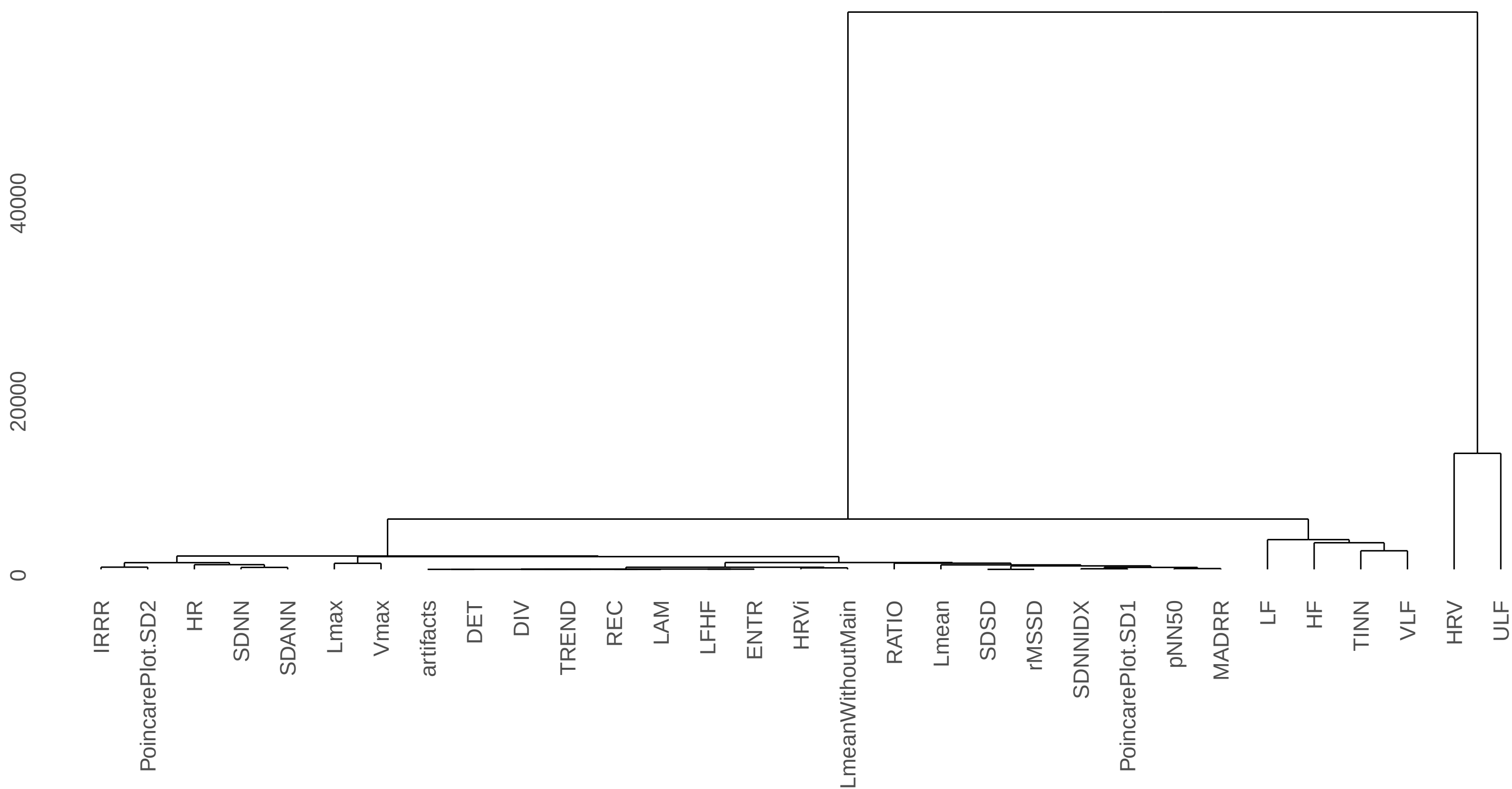
Cluster Dendrogram of all baseline measures using randomly selected days
